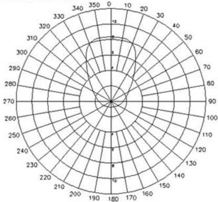
E-PLANE FIELD PATTERNS
