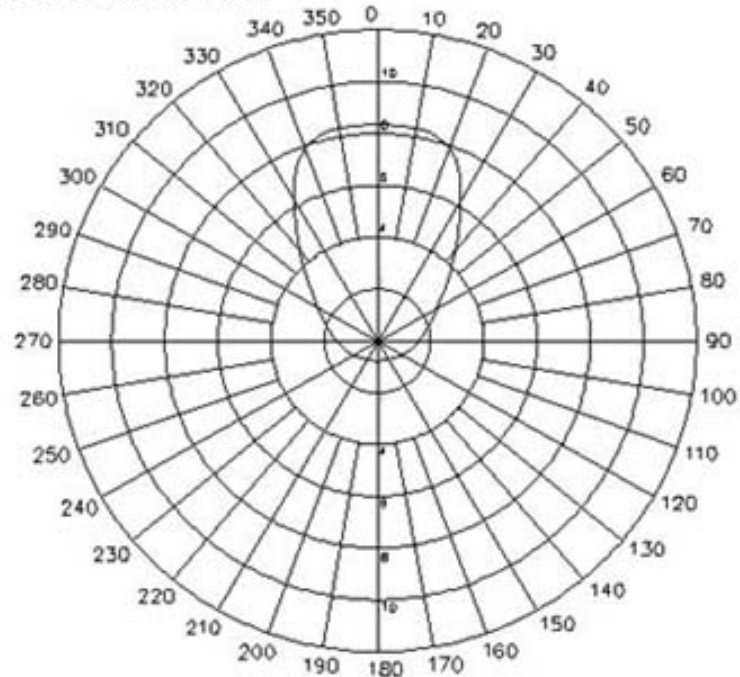
E-PLANE FIELD PATTERNS
